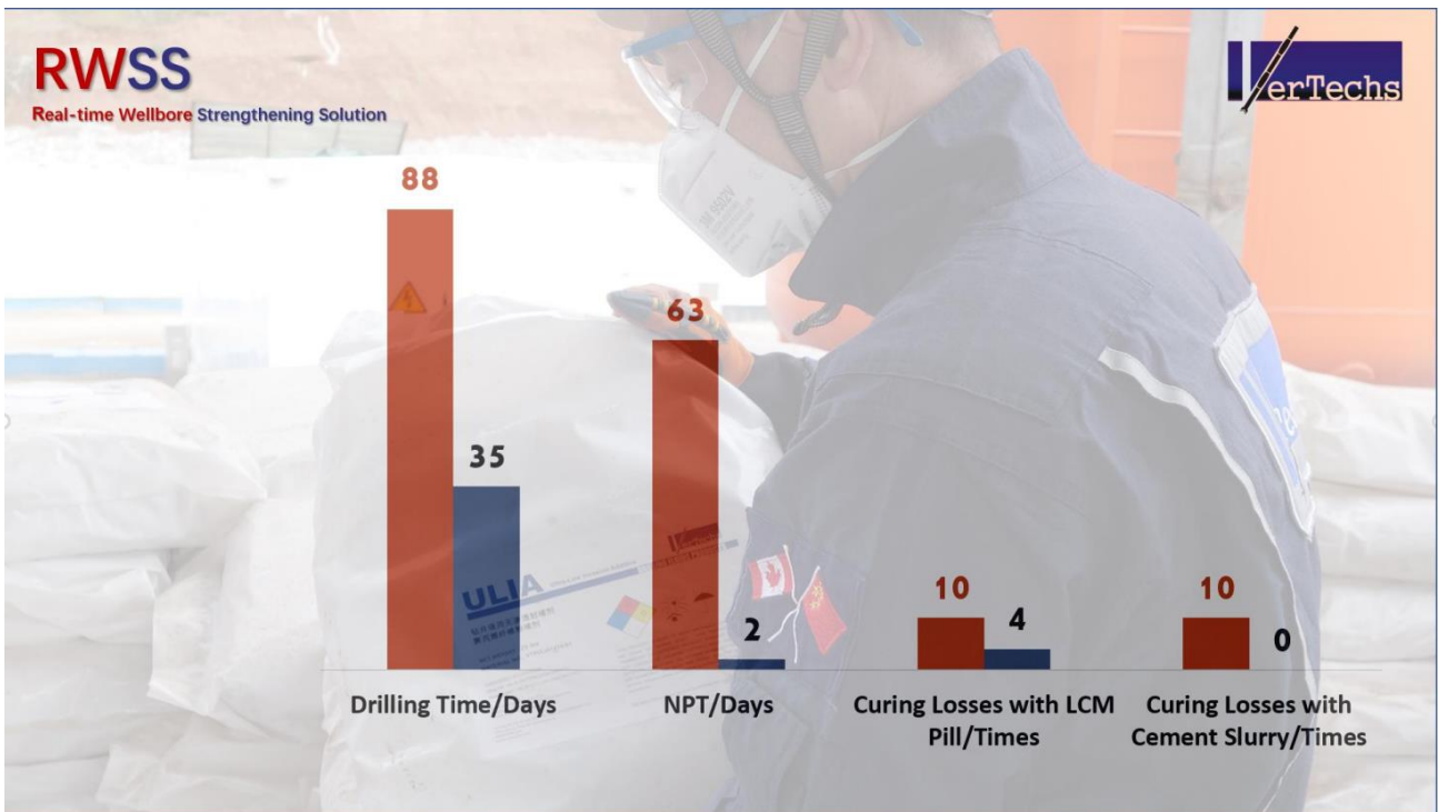
Case Study - An interval drilled with downhole complexity (Red) vs. sidetrack with Vertechs® RWSS (Blue)
